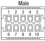
pin layout 10p male connector
