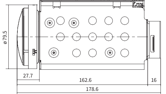
Right
