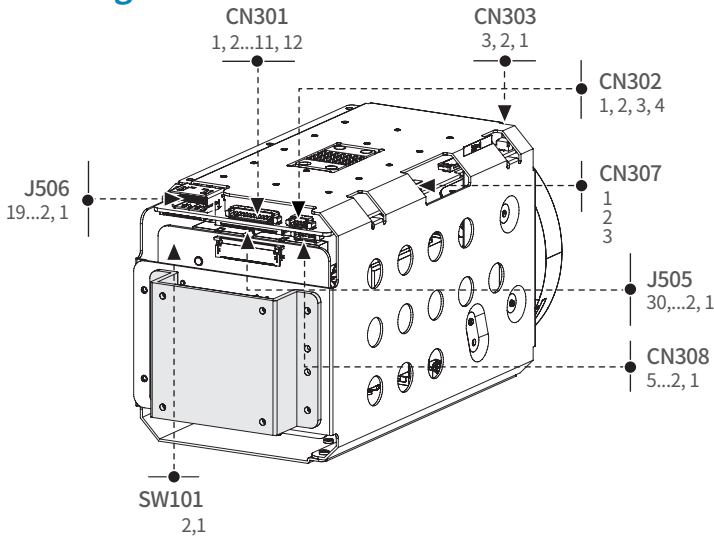
Rear
